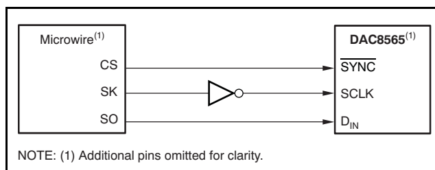
Figure 102. DAC8565 to Microwire Interface
