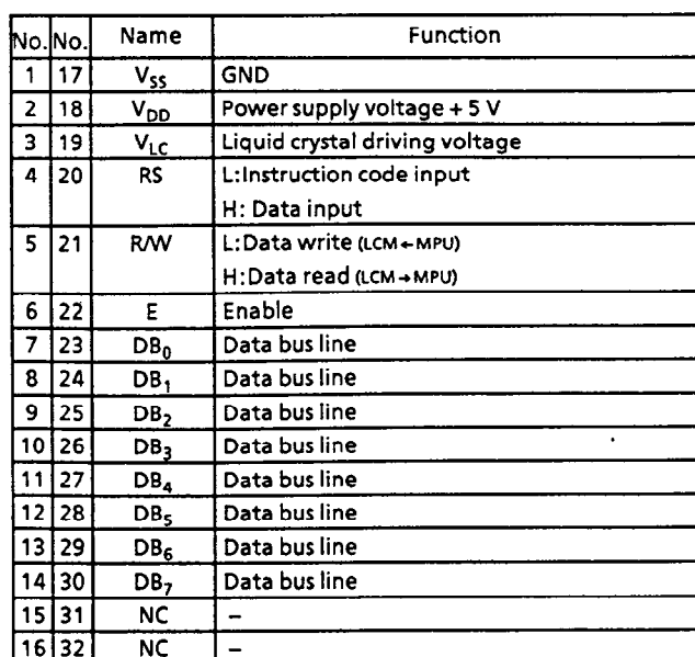
F-3 Pin Functions
