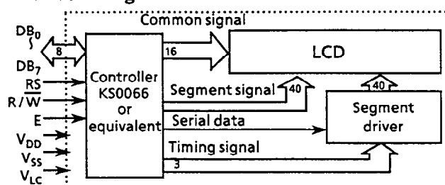
F-4 Block Diagram
