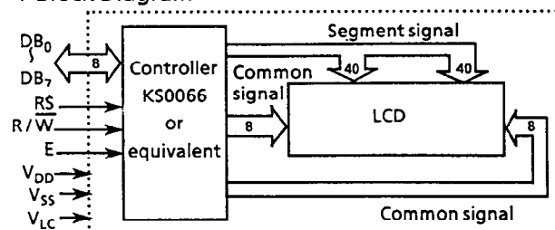
F-4 Block Diagram
