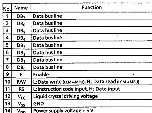
F-3 Pin Functions
