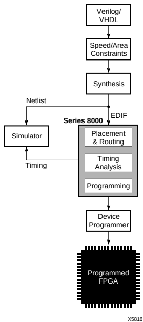
Figure 20: XC8100 Synthesis Design Flow
