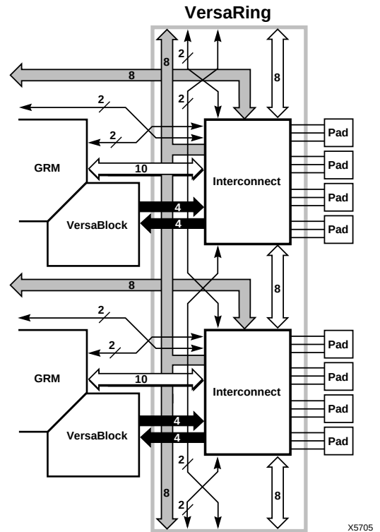
Figure 13: VersaRing I/O Interface
