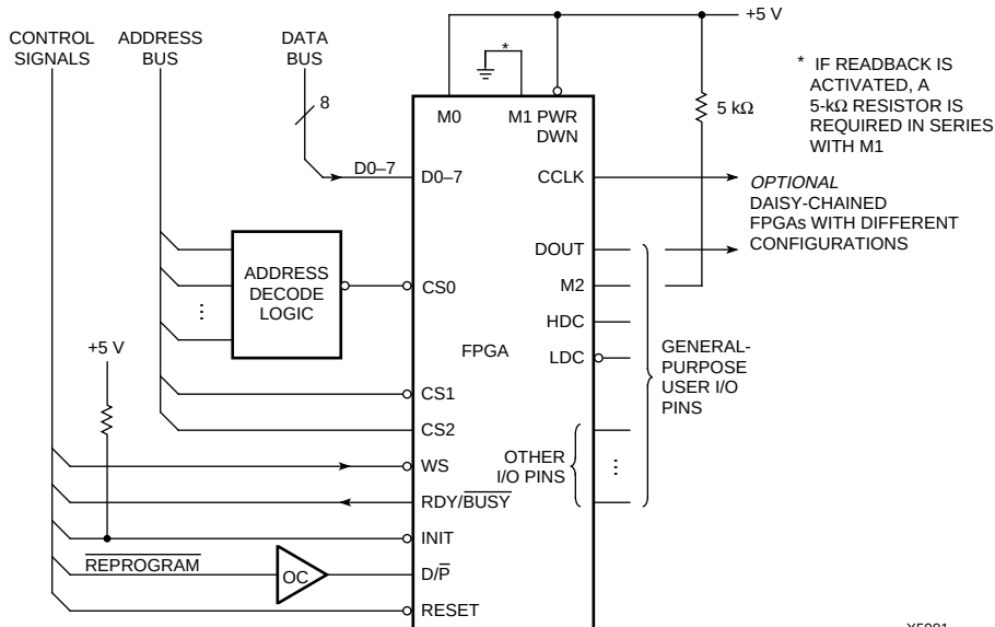
Figure 27: Peripheral Mode Circuit Diagram
