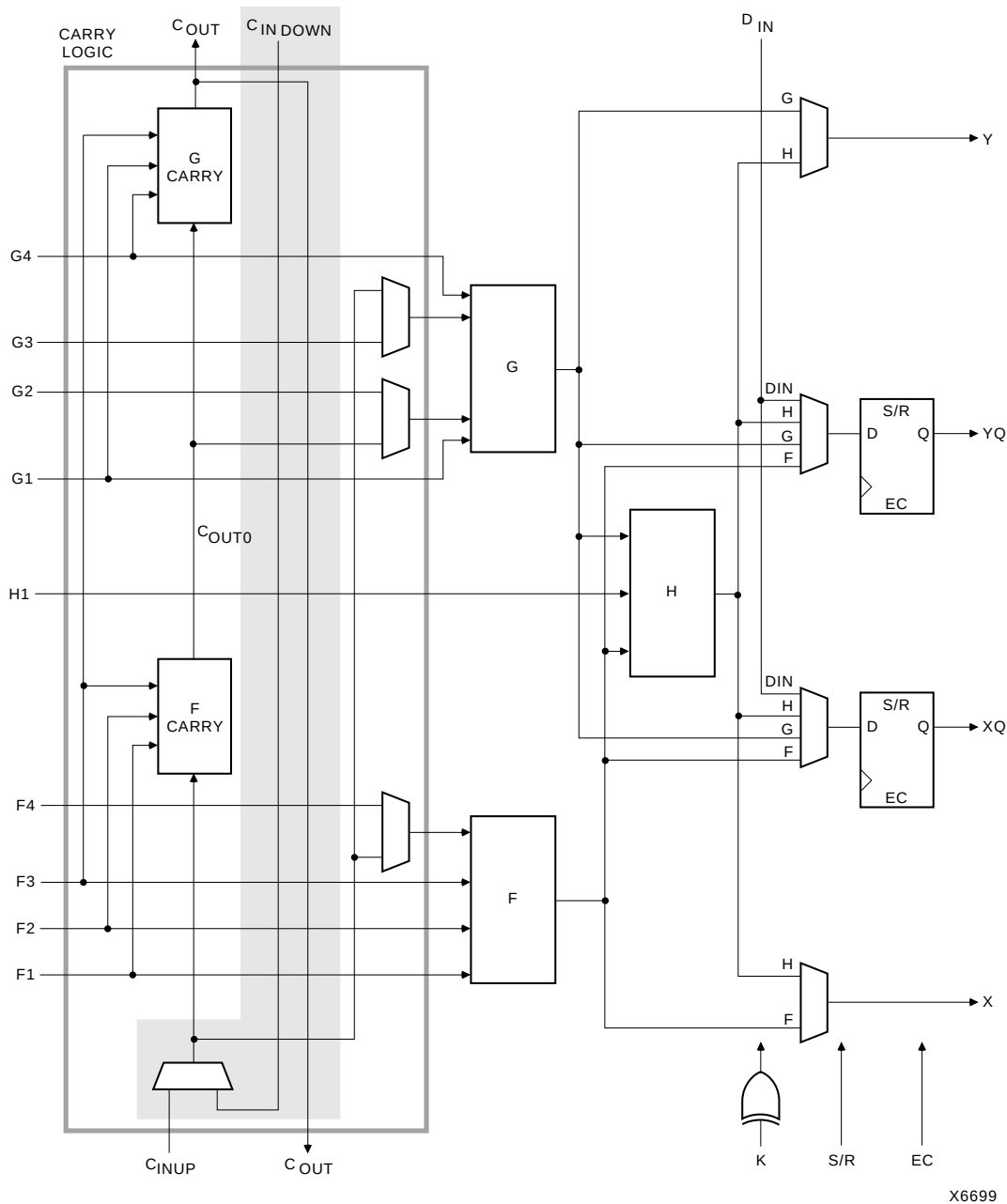
Figure 13: Fast Carry Logic in XC4000E CLB (shaded area not present in XC4000EX)
