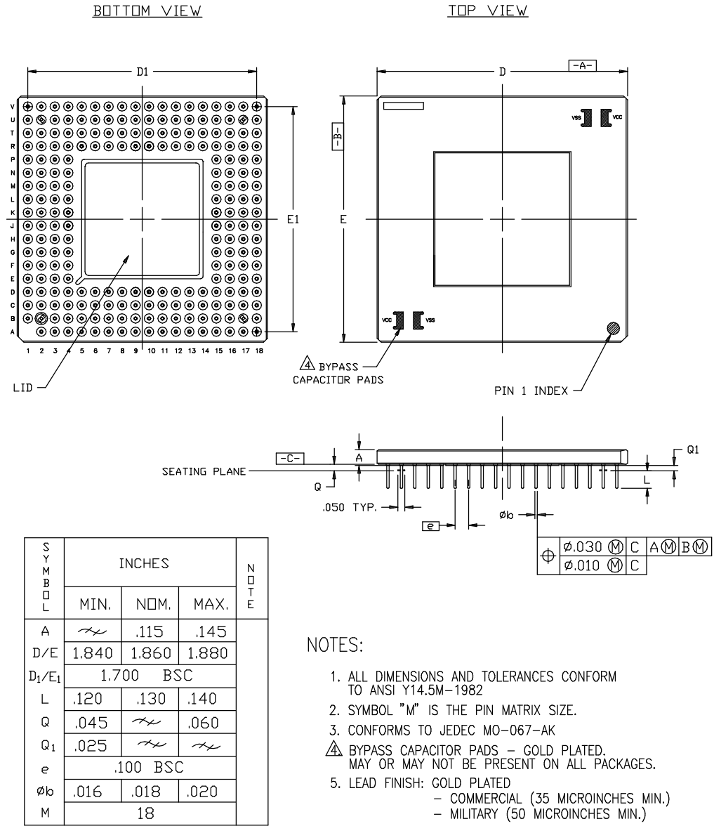
223-PIN CERAMIC PGA (PG223)
