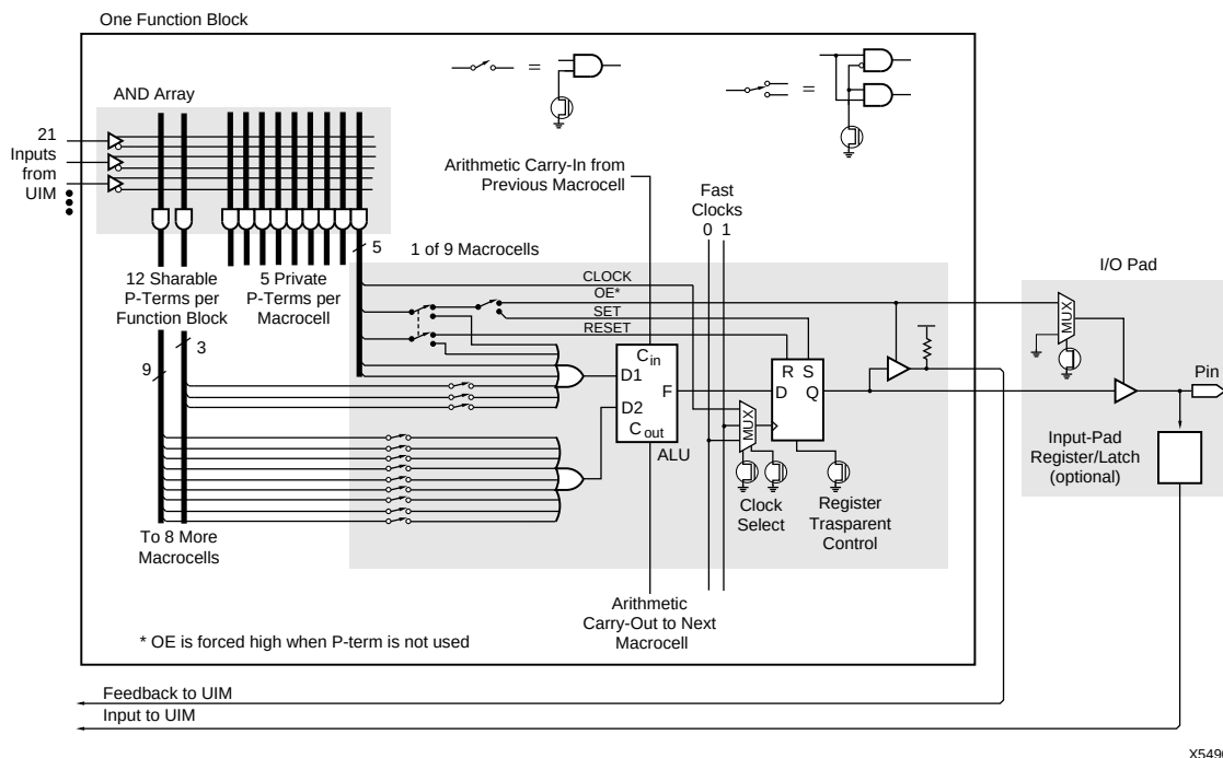
Figure 2: Function Block and Macrocell Schematic
