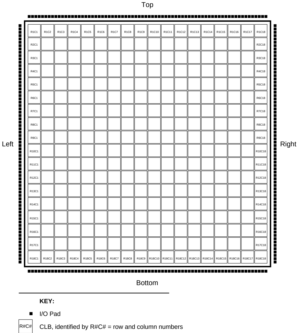
Figure 24: XC5210 CLB-to-Pad Relationship
