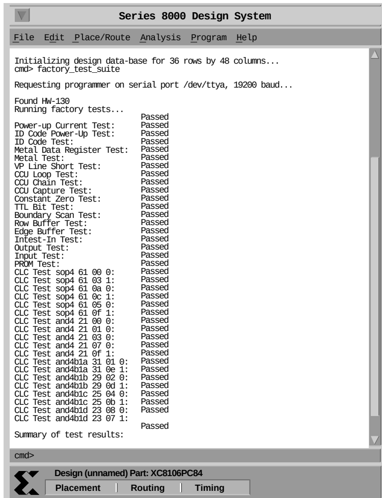
Figure 17: Series 8000 Software Testing a Device in an HW-130
