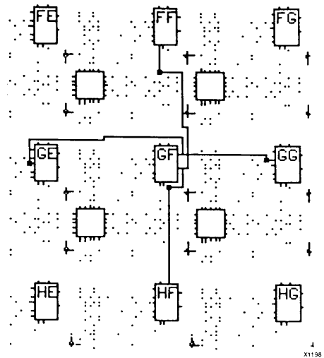
Figure 12: CLB X and Y Outputs.
